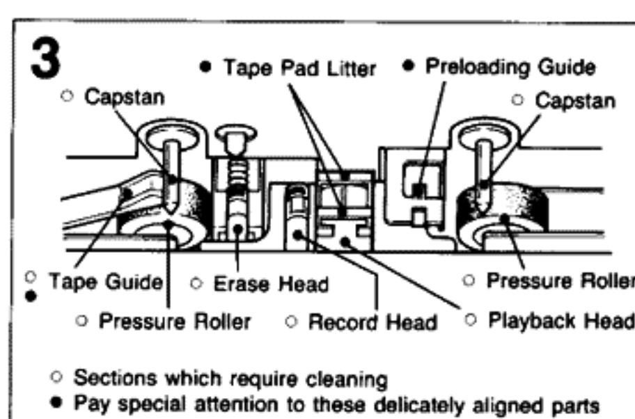
Press the Pause button to release the pressure rollers from the capstans. Now clean the capstans and the surfaces of the heads and tape guides. Finish by using a dry cotton swab, and make sure that no cotton strands are left on any of the cleaned parts.
