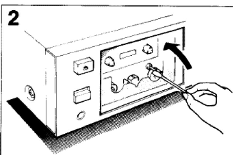
Push the cassette holder back in, switch the deck on and press the Play button. Clean the revolving pressure rollers by holding a cotton swab lightly against the roller on the side turning away from the capstan. Take care that the cotton swab does not get caught between the roller and the capstan.
